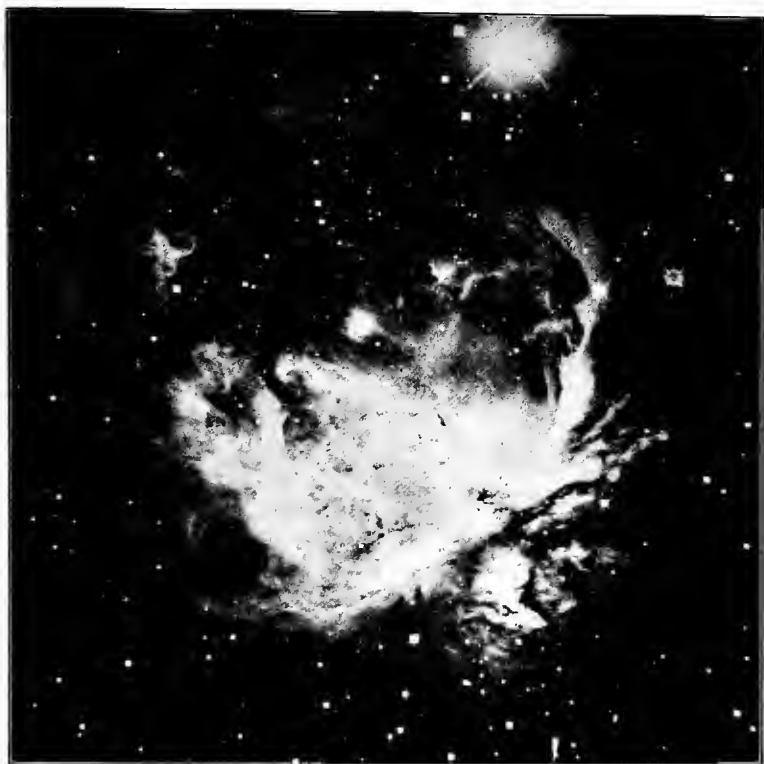
THE ORION NEBULA
